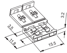
G13286 Connector F080AS, 8mm, white
